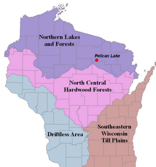
Figure 3.1-2. Location of Pelican Lake within the ecoregions of Wisconsin. After Nichols 1999.
